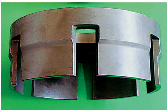
Dog clutch
