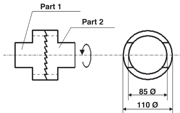
Dog clutch
